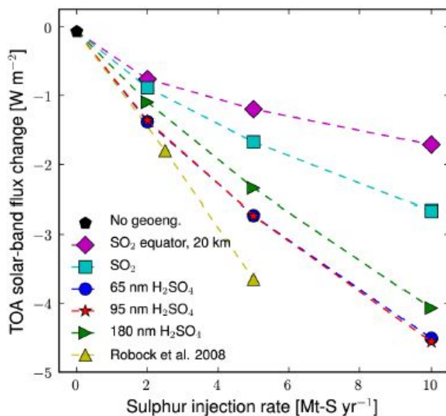
Figure 1: Reduction in incoming top-of-atmosphere (TOA) solar flux achieved for a given yearly dispersal rate. 3
